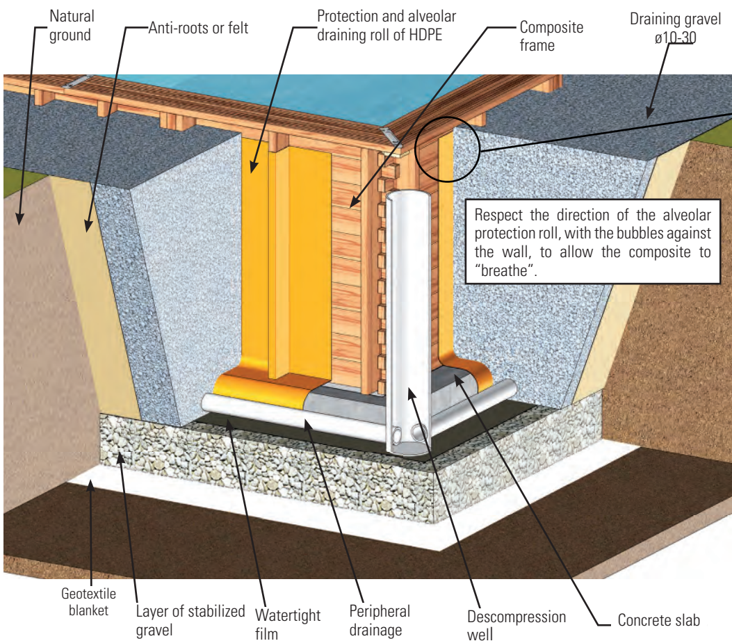
1- Composite frame 2- Roll of alveolar protection an drainage of HDPE
